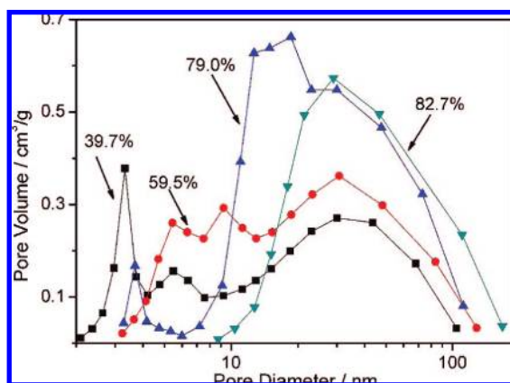
Figure 5. Pore structures developed after different levels of ammonia desorption from a \text{Mn}(\text{NH}_3)_6\text{Cl}_2 tablet.
